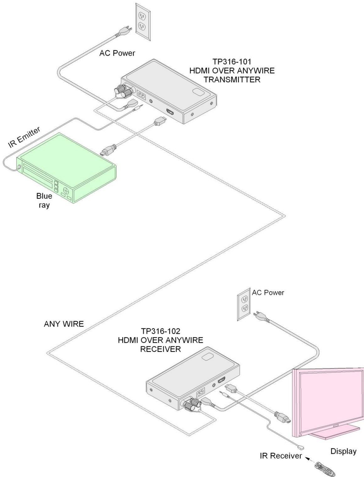
Diagram 1: Typical Setup
